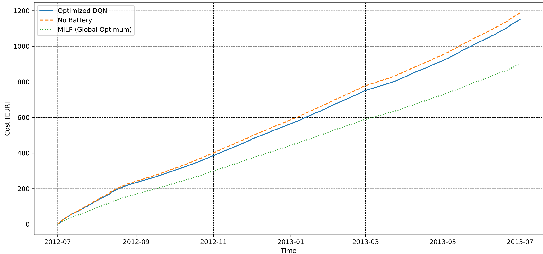
User 172 - Basic Training - Electricity Cost [DQN vs MILP]
